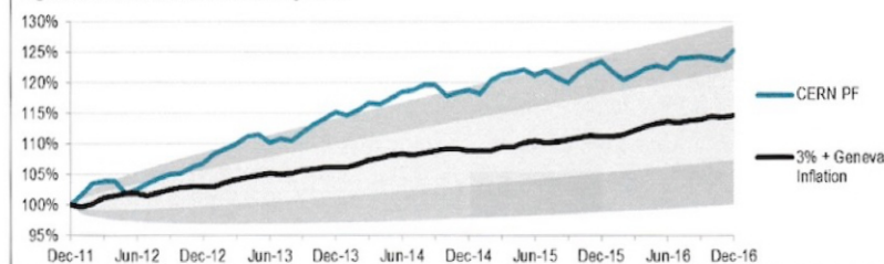
Figure 1: Cumulative Return vs. Objective
